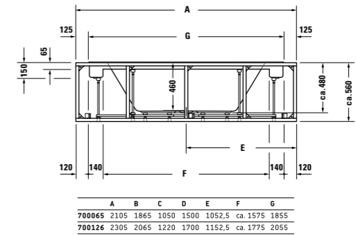
# 700065 00 0 00 0000, 2000 x 1000 mm + # 790831 00 0 00 0000, Auffaltbares Ruhedeck. Relaxations deck. Copertura imbottita pieghevole. Banquette de relaxation. Inklapbaar zonedek. Tumbona plegable + # 790153 00 0 00 0000, Schienensystem. Rail-mount system. Sistema a binari. Système de rails. Railmodule. Sistema de perfiles # 700126 00 0 00 0000, 2200 x 1000 mm + # 790848 00 0 00 0000, Auffaltbares Ruhedeck. Relaxations deck. Copertura imbottita pieghevole. Banquette de relaxation. Inklapbaar zonedek. Tumbona plegable + # 790154 00 0 00 0000, Schienensystem. Rail-mount system. Sistema a binari. Système de rails. Railmodule. Sistema de perfiles Einbauversion. Built-in. Versione da incasso. Version à encastrer. Inbouwversie. Versión empotrada
